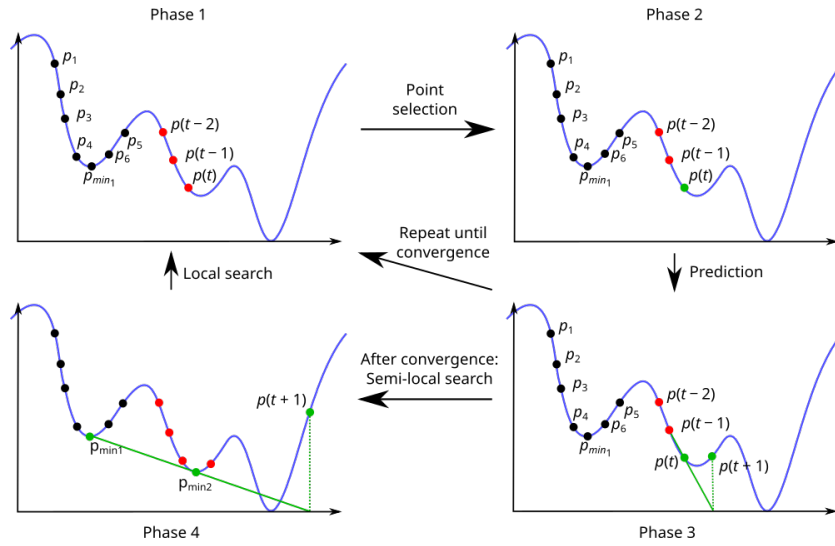
Fig. 1. The search phases of CoBOpt: point selection, local search, higher level search
