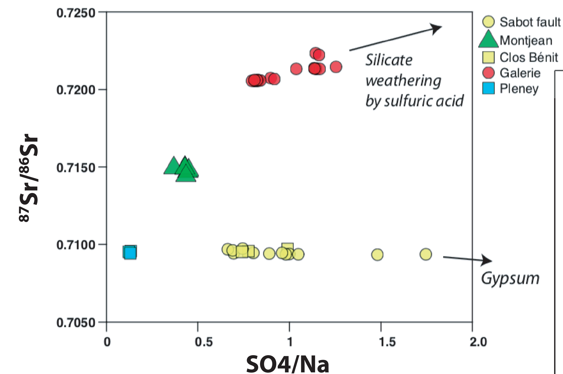
FIG 6 : \text{SO}_4/\text{Na} VS ^{87}\text{Sr}/^{86}\text{Sr} - FOR THE DIFFERENT SAMPLED SOURCES : GALERIE = G710 + C79 ; SABOT FAULT = FONAFFREY + BATHIE + THIEBAUDS + MATHIEUX ; PLENEY ; CLOS BENIT (WHICH IS CLOSE TO SABOT FAULT SOURCES)
