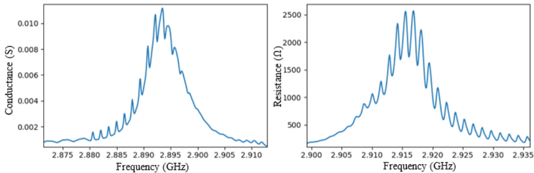
Fig. 12. Example of series (a) and parallel (b) resonances of the pseudo-BAW mode for a device with e_{AlN}/p = 0.7 exhibiting strong contributions from bulk resonances of the substrate.
