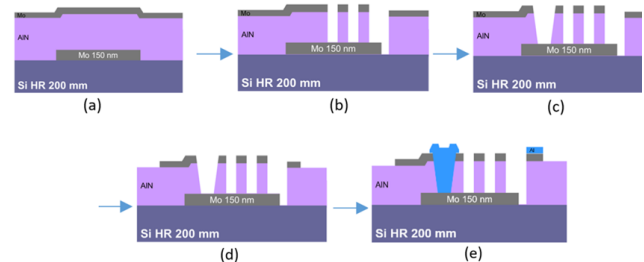
Fig. 2. Five mask process flow for the fabrication of hybrid SAW/BAW resonators: (a) patterning the bottom electrode and deposition of AlN and Mo, (b) patterning the top electrode and the AlN film to form the transducers, (c) opening vias through the AlN layer for electrical contact towards the bottom electrode, (d) patterning the top electrode, (e) Al pads deposition using lift-off.
