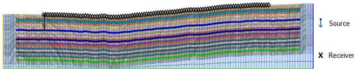
Fig. 6. Interface model consisting of 28 layers and 29 interfaces with a length of 126 m and a depth of 23.5 to 31 m. We have 96 receivers in total and 1 source located at the free surface. The dominant source frequency is 80 Hz and the source type is Gaussian. The total number of time steps is 60000 and the time step of recording is 0.0000125 s. The element size is around 1 m. The P and S seismic velocities are from 640 up to 3900 m/s and from 370 up to 2200 m/s respectively.
