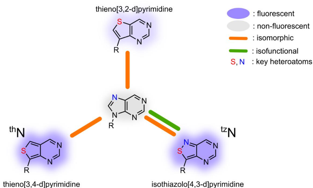
Figure 7. Three classes of isomorphic emissive purine analogues resulting from chemical mutagenesis of the natural purine (in the centre). R = ribose or 2'-deoxyribose (Adapted from 199,201 ).
