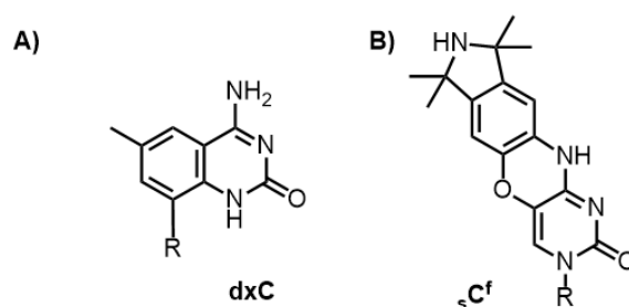
Figure 31. Chemical structures of the benzo-expanded cytosine dxC (A) and sC f (B). R = 2'-deoxyribose.
