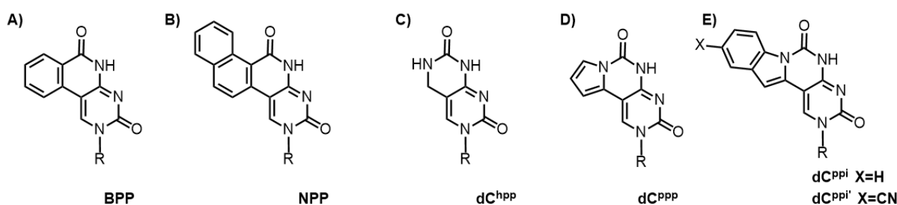
Figure 30. A) Benzopyridopyrimidine ( BPP ), B) Naphthopyridopyrimidine ( NPP ). C-E) Fluorescent cytosine analogues synthesized by the group of Sekine; R = 2'-deoxyribose.
