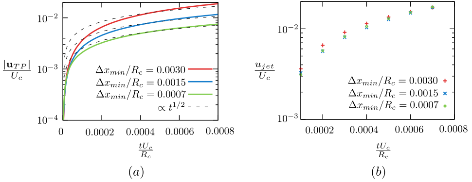
Figure 10: The grid convergence of viscous solution (a) The evolution of velocity of contact line is plotted for different grid-size. (b) The evolution of jet velocity is plotted for various grid size.
