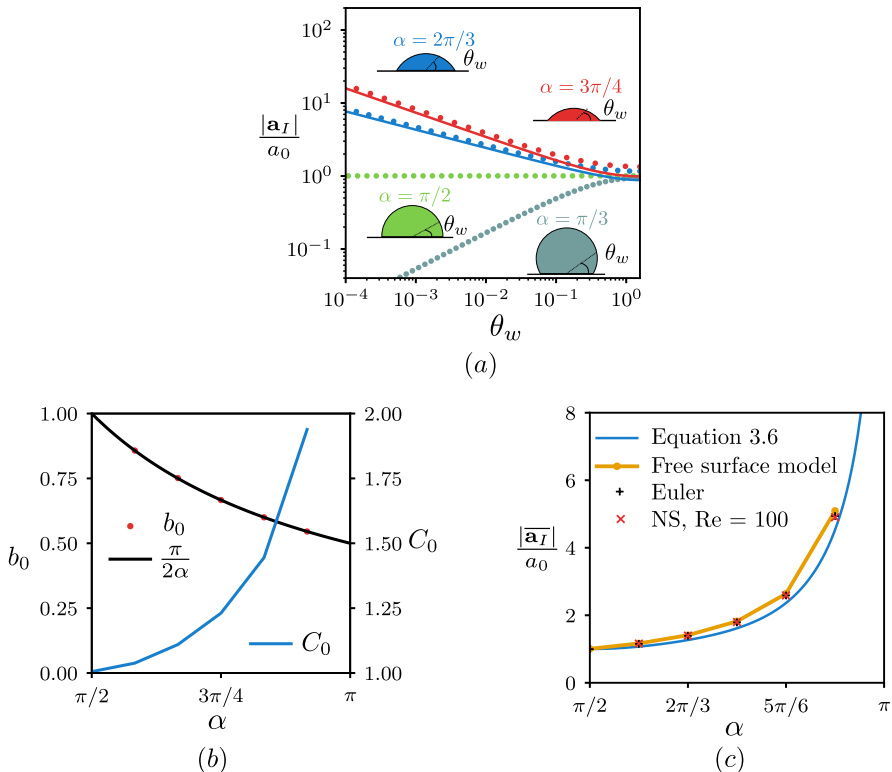
Figure 3: (a) Non-dimensional acceleration magnitude, |a_I|/a_0 along the interface parametrised using the angle \theta_w (measured in the counter-clockwise direction from the point of contact of wall and the axis of symmetry) for \alpha = \frac{\pi}{3}, \frac{\pi}{2}, \frac{2}{3}\pi, \frac{3}{4}\pi . Dots represent the numerical solution from free surface model and the thick lines are predictions using equation 3.4 evaluated at the interface. (b) Exponent b_0 and coefficient C_0 obtained from the free surface model along the wall for different \alpha . (c) Non-dimensional averaged interface acceleration magnitude as a function of the contact angle using different methods: analytical expression given by equation 3.6 (blue line), the solution from the free surface model (yellow line), the DNS solution of the Euler equations (black crosses), and the DNS solution of the Navier–Stokes solver for Re = 100 (red crosses).
