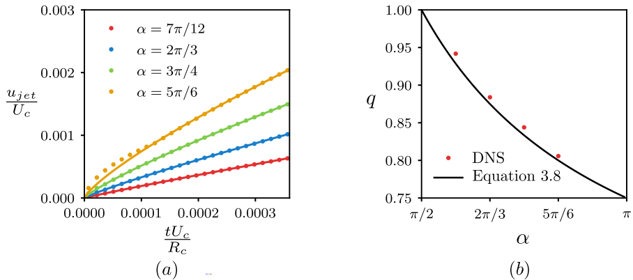
Figure 5: (a) Evolution of jet velocity for different contact angles from (dots) DNS and (solid lines) fitting using equation 3.7. (b) Exponent q from DNS fitting and predictions of equation 3.8.
