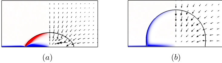
Figure 6: The vorticity is shown in colour map and velocity vectors obtained from DNS after short time short time ( \frac{tU_c}{R_c} = 0.1 ) for \text{Re} = 100 for (a) \alpha = 2\pi/3 and (b) \alpha = 5\pi/12 .
