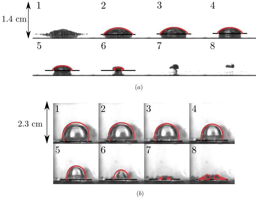
Figure 7: The snapshots of bubble shape are shown for the two representative cases, the numerical bubble shapes shown with red curves are overlaid at same times and scaled to same length as in experiments. (a) Case where \alpha > \pi/2 , each snapshots are taken every 0.1 ms (b) Case where \alpha < \pi/2 , each snapshots are taken every 0.125 ms.
