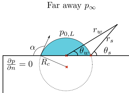
Figure 1: Problem setup and different coordinate systems used in this article i.e. (r_w, \theta_w) and (r_s, \theta_s)
