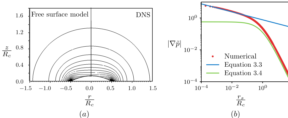
Figure 2: (a) Isocontours of the magnitude of acceleration for bubble with \alpha = \alpha = 3\pi/4 : The isocontours in the left half are obtained from free surface model and those in the right half are obtained from DNS. (b) Non-dimensional acceleration magnitude along the wall obtained for bubble with \alpha = 3\pi/4 using the free surface model.
