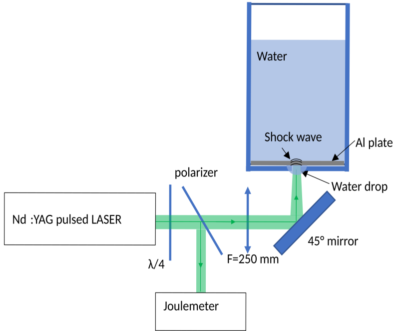
Figure 11: Experimental setup used to create flat bubbles.
