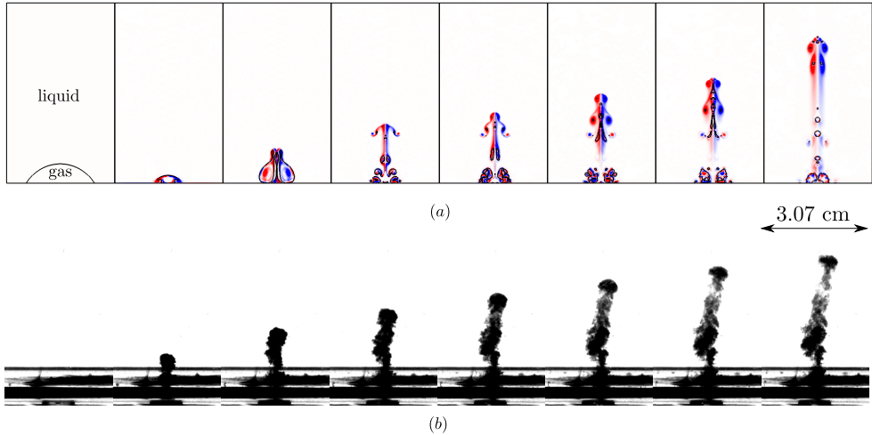
Figure 8: (a) Bubble interface in black curve and the vorticity field in the colour map as obtained from DNS is shown at (consecutively from left to right) \frac{tU_c}{R_c} = 0, 0.19, 0.3, 0.81, 1.00, 1.45, 1.95, 4.90 . An the annular jet parallel to wall reaches the axis resulting in to the jet directed away from the wall which later generates the vortex ring. The results are plotted for \alpha = 2\pi/3 and Re = \infty We = \infty (b) The visualisation of liquid flow field obtained by adding dye at the bottom of tank resulting from collapse of bubble is shown at every 2.5ms.
