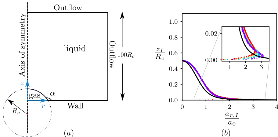
Figure 4: (a) The numerical setup for DNS (b) Results from the DNS for \alpha = 2\pi/3 and Re = 100 . Time averaged interface acceleration in direction parallel to the wall, a_{r,I} = u_{r,I}/t , as a function of the distance from the wall (in colour where tU_c/R_{c,0} \in [7.27 \cdot 10^{-5}, 3.6 \cdot 10^{-4}] ). For reference we include the potential flow solution given by equation 3.4 evaluated at the interface (solid black line). The inset represents a zoom in to the viscous boundary layer generated close to the wall.
