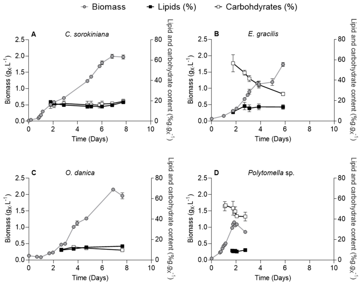
Figure 6: Carbohydrates and lipids production by candidate strains on synthetic DFE. The figures represent biomass dry weight ( \text{g}\cdot\text{L}^{-1} , grey circles) and product content in each strain ( \%g\cdot g^{-1} , carbohydrates in white squares and lipids in black squares) evolution as a function of time (days) in (A) C. sorokiniana SAG, (B) E. gracilis , (C) O. danica and (D) Polytomella sp. cultures. Strains were cultivated in flasks in synthetic medium ( 0.3\text{ gcs}\cdot\text{L}^{-1} acetate (Ac) and 0.7\text{ gcs}\cdot\text{L}^{-1} butyrate (Bu); pH 7) under constant illumination and shaking. All data are given as mean and standard deviation of three biological replicates. Lack of data points in early phase indicates a product concentration below quantification limit due to lack of sufficient biomass.
