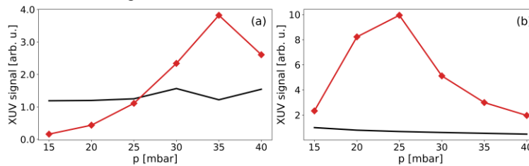
Fig. 2. Signal of the 19 th harmonic in Kr without (black) and with 8% pre-ionization (red) (a). H19 signal from rigorous numerical simulations without (black) and with the pre-ionization (red) (b).
