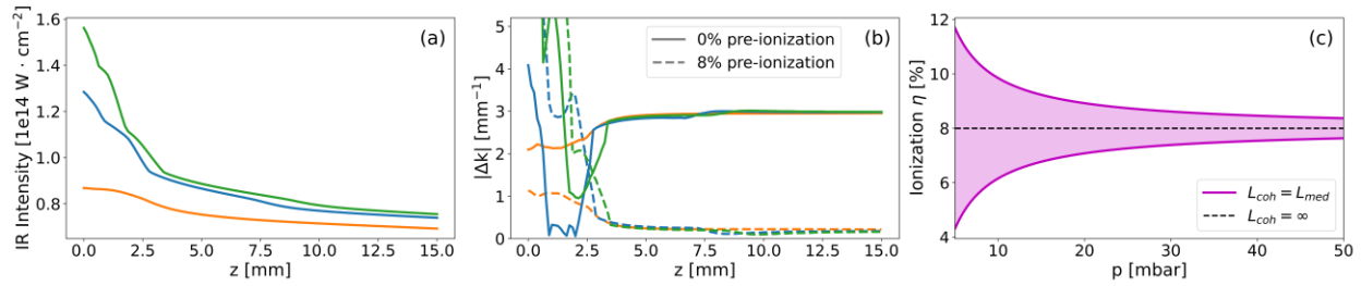
Fig. 1. (a) Evolution of on-axis intensity for different pulse intensities at the entrance of a 15-mm long medium with 36 mbar of Kr. (b) Comparison of phase-mismatch for the same pulses as in (a) and 19 th harmonic for situation without pre-ionization (full lines) and with 8% pre-ionization (dashed lines). (c) Optimal degree of ionization for 19 th harmonic generated by 800 nm laser in krypton as a function of pressure in 15-mm long medium.
