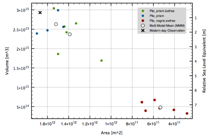
Figure 7. Ice sheet volume [ \text{m}^3 ] and area [ \text{m}^2 ] of Pliocene scenarios \text{Plio}_{\text{prism.icefree}} (green), \text{Plio}_{\text{prism}} (blue), and \text{Plio}_{\text{nogris.icefree}} (red) with relative sea level equivalent [m] with respect to present-day reconstructions. Cross denotes volume and area for Bamber et al. (2001a), open circles indicate multi-model means (MMM) for the respective scenarios.
