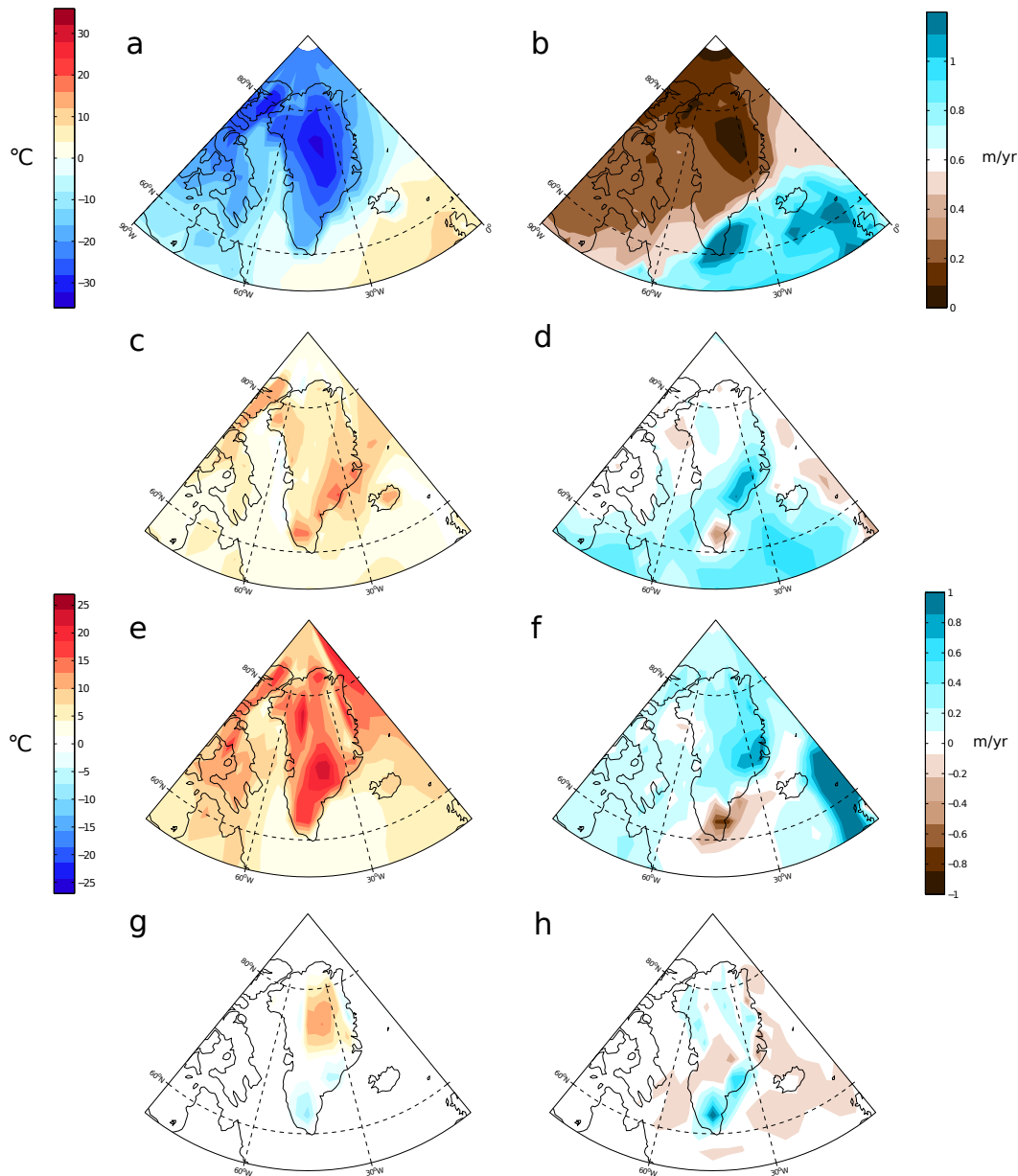
Figure 1. Control and Pliocene Phase driving climatologies. Annual surface temperatures [ ^{\circ}\text{C} ] and precipitation [ \text{m yr}^{-1} ] for (a–b) Had ctrl , (c–d) NCEP2 ctrl – Had ctrl differences, (e–f) Had prism – Had ctrl differences, and (g–h) Had plio.nogris – Had prism differences. Note change in scales for absolute (a–b) and difference calculations (c–h).
