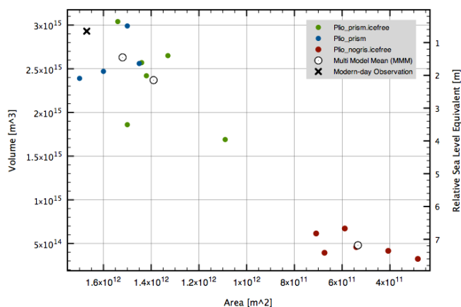
Figure 7. Ice sheet volume [ \text{m}^3 ] and area [ \text{m}^2 ] of Pliocene scenarios \text{Plio}_{\text{prism.icefree}} (green), \text{Plio}_{\text{prism}} (blue), and \text{Plio}_{\text{nogris.icefree}} (red) with relative sea level equivalent [m] with respect to present-day reconstructions. Cross denotes volume and area for Bamber et al. (2001a), open circles indicate multi-model means (MMM) for the respective scenarios.
