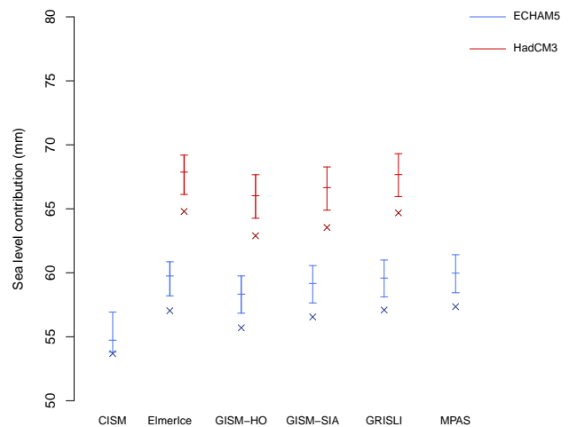
Fig. 1. Projected cumulative GrIS sea level contributions for the ECHAM5 and HadCM3 A1B projections at 2100. Crosses mark simulations with no elevation feedback. Bars mark the estimated 95 % credibility intervals and (central tick) best estimates of the elevation feedback parameterisation.
