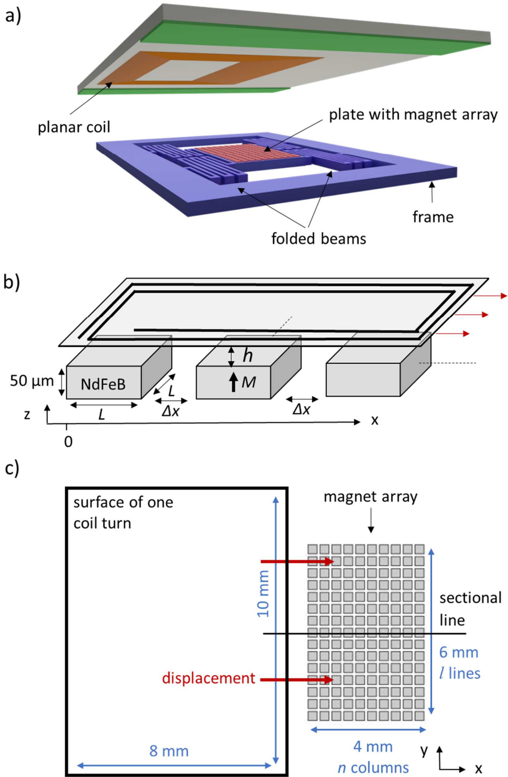
Figure 1: (a) Design of the vibrating energy harvester considered here. The vibrating plate is connected to the frame by 4 folded beams (each containing 3 folds). The magnetic array is on the 6 \times 4\ \text{mm}^2 vibrating plate and centred with respect to the turns on one side of the facing planar coil. (b) Schematic view of 50\ \mu\text{m} -thick NdFeB cuboids constituting the (xy) magnet array with out-of-plane magnetization. Cuboids have a lateral dimension of L and interspacing of \Delta x , (c) Geometry considered in the simulation: a 10 \times 8\ \text{mm}^2 surface, representing one coil turn, is displaced above the 6 \times 4\ \text{mm}^2 magnet array constituted of n columns and l lines.
