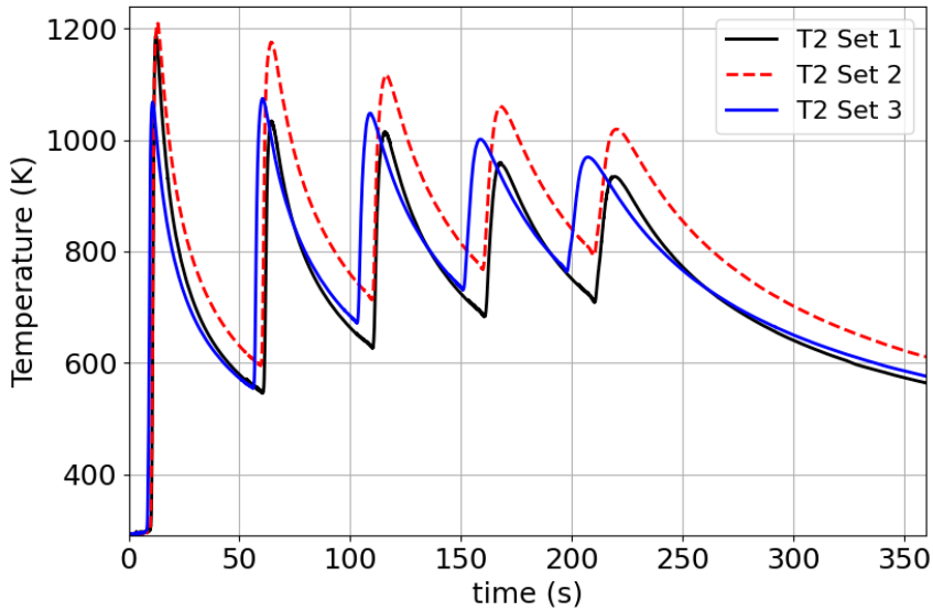
Figure 13: T2 thermal cycles for the three sets of process parameters along the deposition of 5 layers.
