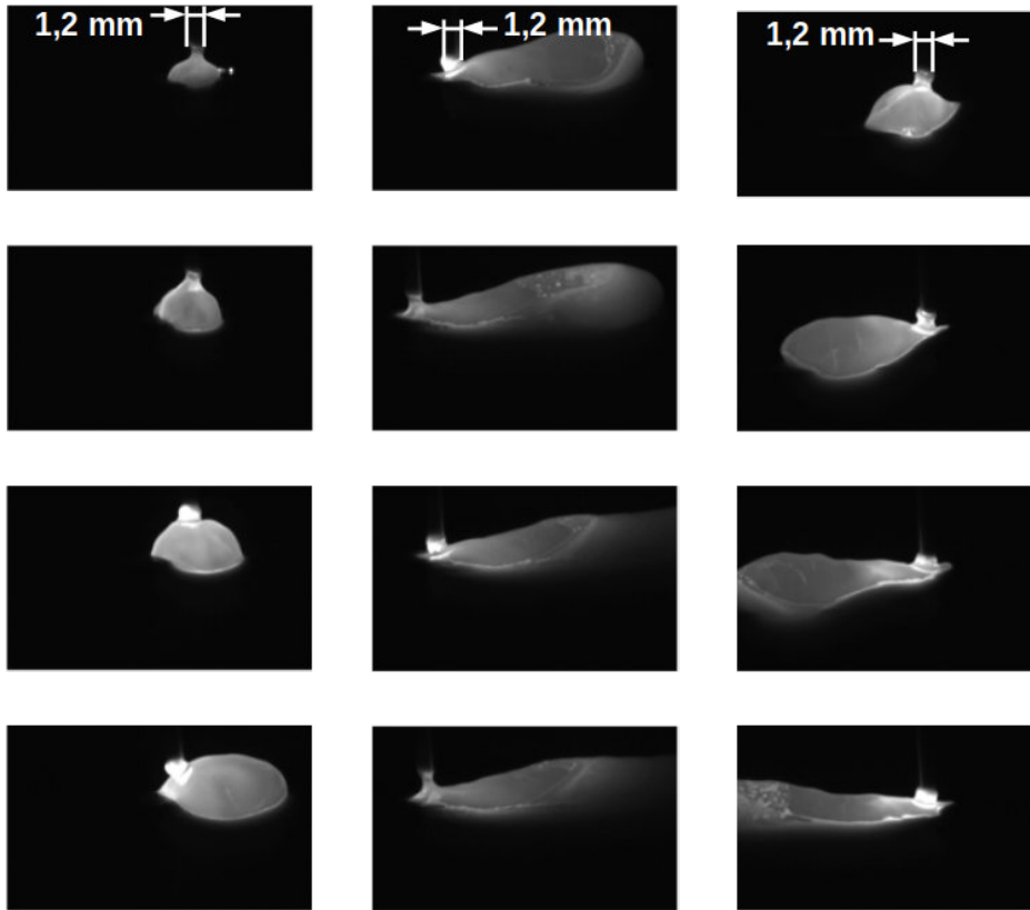
Figure 3: Images obtained with the camera located on the side of the welding torch during the deposit of melted wire: initiation of weld pool for the first layer (1st column), during the 1st layer (2nd column) and for the 2nd layer (3rd column). Experiment was realized with #S1 set of parameters (for dimension indication, the diameter of the feed wire is 1.2 mm).
