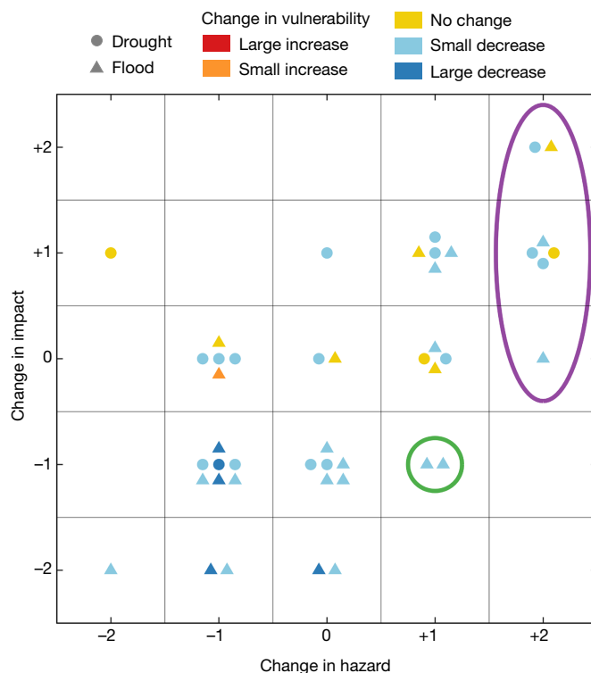
Fig. 3 | Relationship between change in hazard and change in impacts. Categories are: lower hazard and lower impact, ten cases; higher hazard and higher impact, 11 cases; lower hazard and higher impact, one case; higher hazard and lower impact, two cases. Circles and triangles indicate drought and flood paired events, respectively; their colours indicate change in vulnerability. Green circle highlights success stories ( n = 2 ) of reduced impact (-1) despite a small increase in hazard (+1). Purple ellipse indicates paired events ( n = 7 ) with large increase in hazard (+2)—that is, events that were subjectively unprecedented and probably not previously experienced by local residents.
