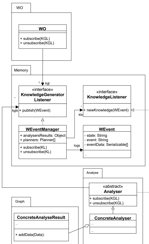
Figure 6: Static model of Monitor, Analysis & Knowledge
