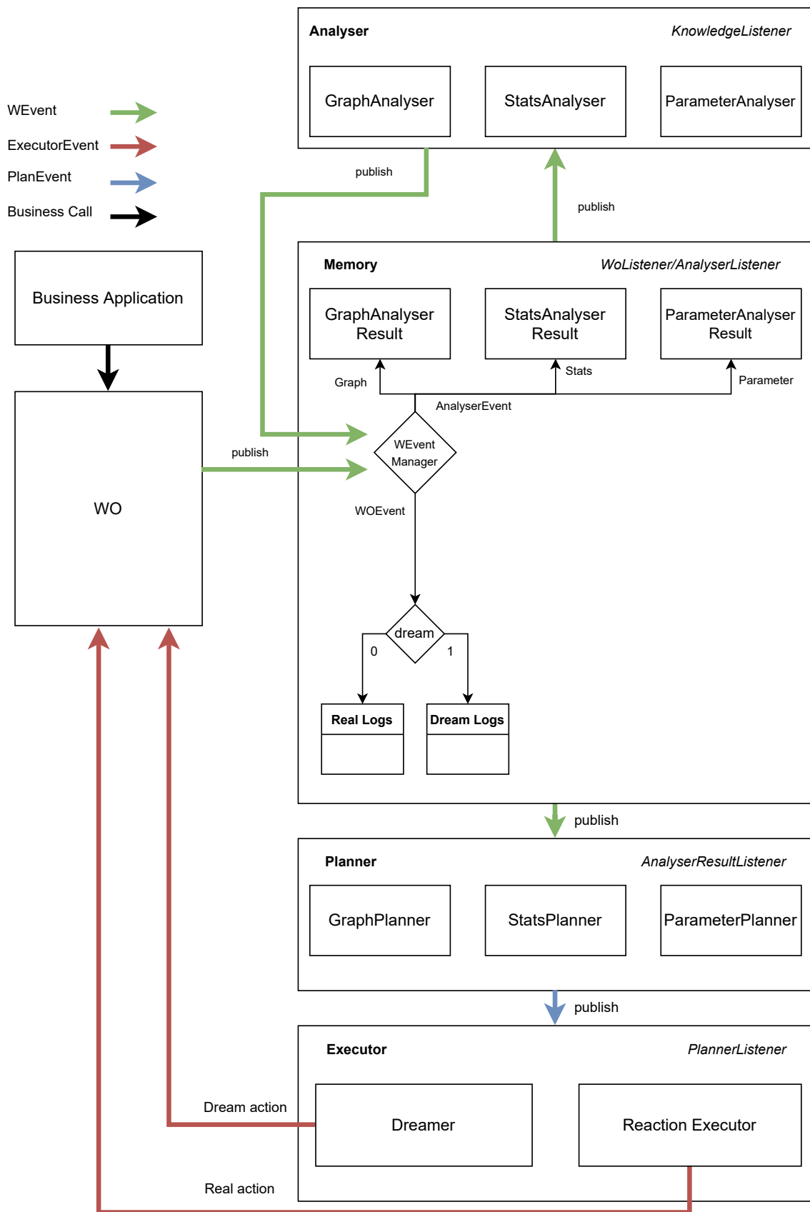
Figure 4: Meta-model of the new architecture
