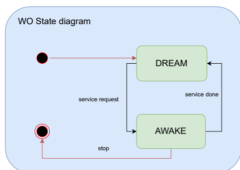
Figure 3: Original WO high-level states
