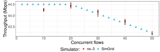
Figure 3: Throughput degradation under concurrent flows.
