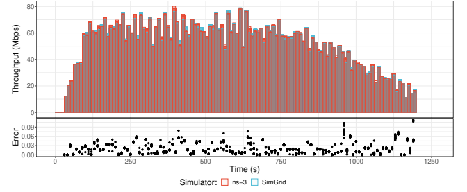
Figure 9: On top, data received by the gateway node by 10s intervals with 22 cells and 126 stations. In the bottom, relative error between ns-3 and SimGrid
