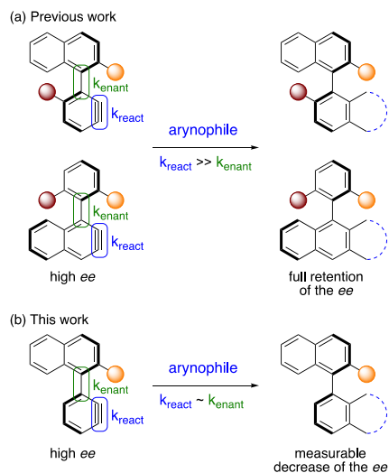
Scheme 1. Aryne Atropisomers With a 1-Phenylnaphthalene Backbone; (a) Conformationally Stable Aryne Atropisomers (ref 9); (b) Conformationally Labile Aryne Atropisomer
