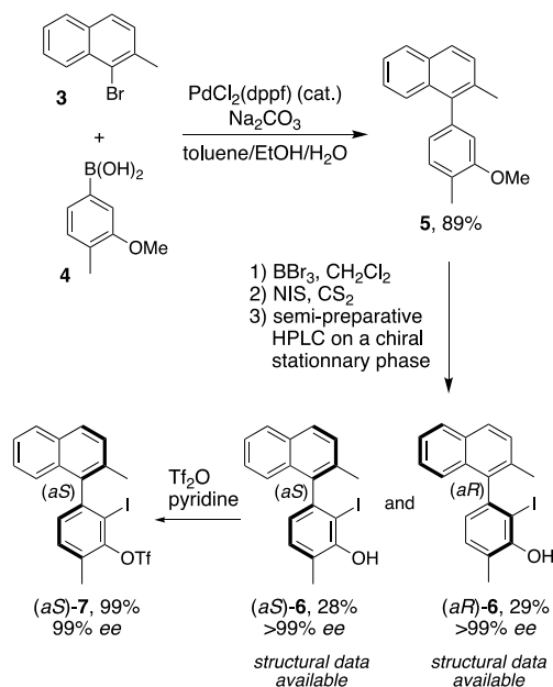
Scheme 2. Synthesis of the Aryne Atropisomer Precursor ( aS )- 7 a
