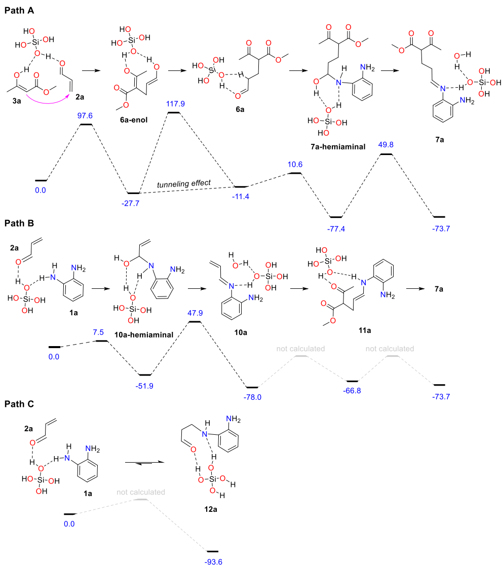
Scheme 3. Energy profile of both mechanistic scenarios leading to 7a (paths A and B) and relative energy of the aza-Michael adduct 12a (path C). All energies are Gibbs free energies expressed in kJ·mol -1 at 298 K.
