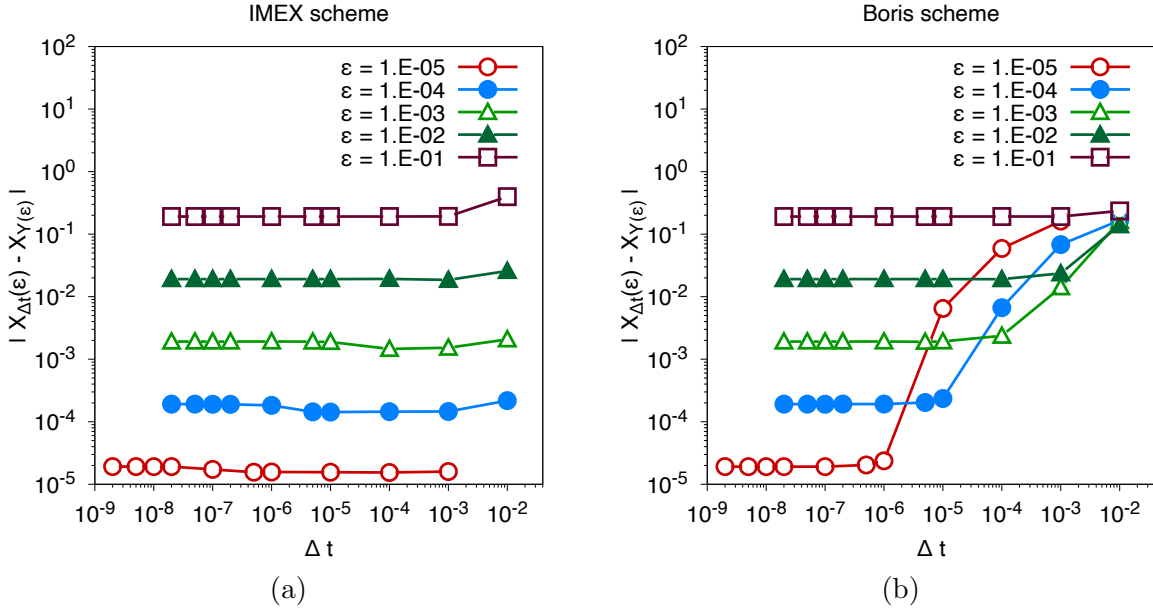
FIGURE 2. Particle motion without electric field. Numerical errors \|\mathbf{X}_{\Delta t}(\epsilon) - \mathbf{X}_{\mathbf{Y}(\epsilon)}\| , \mathbf{X}_{\mathbf{Y}(\epsilon)} being the spatial position built from \mathbf{Y} , obtained for different \epsilon with (a) second order scheme (4.10)-(4.12) and (b) the Boris scheme [2], plotted as functions of \Delta t .
