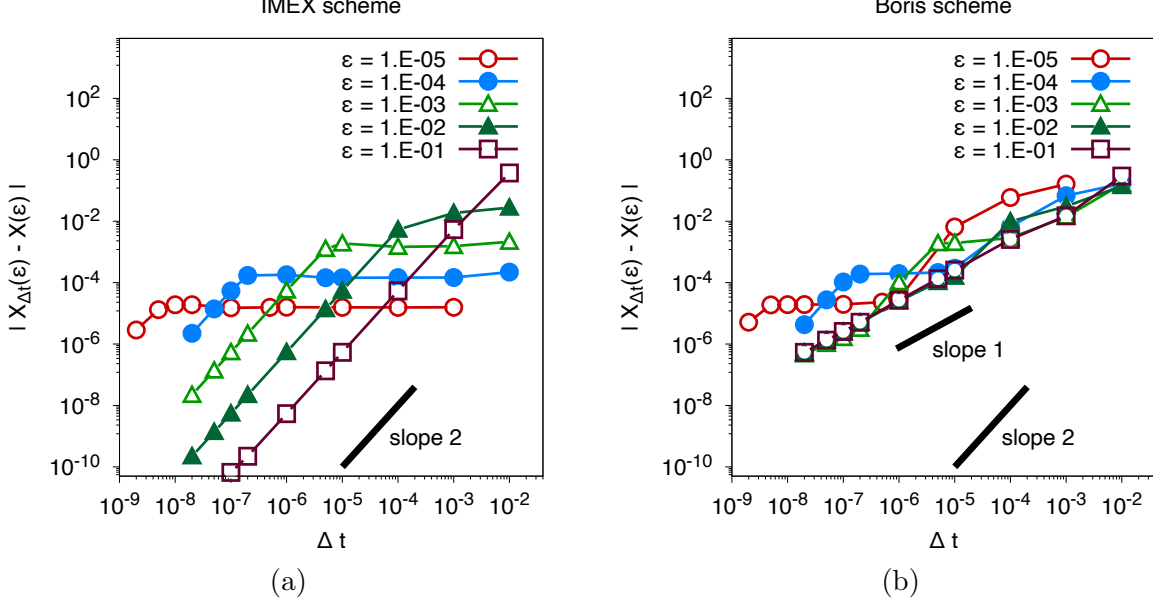
FIGURE 1. Particle motion without electric field. Numerical errors \|\mathbf{X}_{\Delta t}^\epsilon - \mathbf{X}^\epsilon\| obtained for different \epsilon with (a) the second order scheme (4.10)-(4.12) and (b) the Boris scheme [2], plotted as functions of \Delta t .
