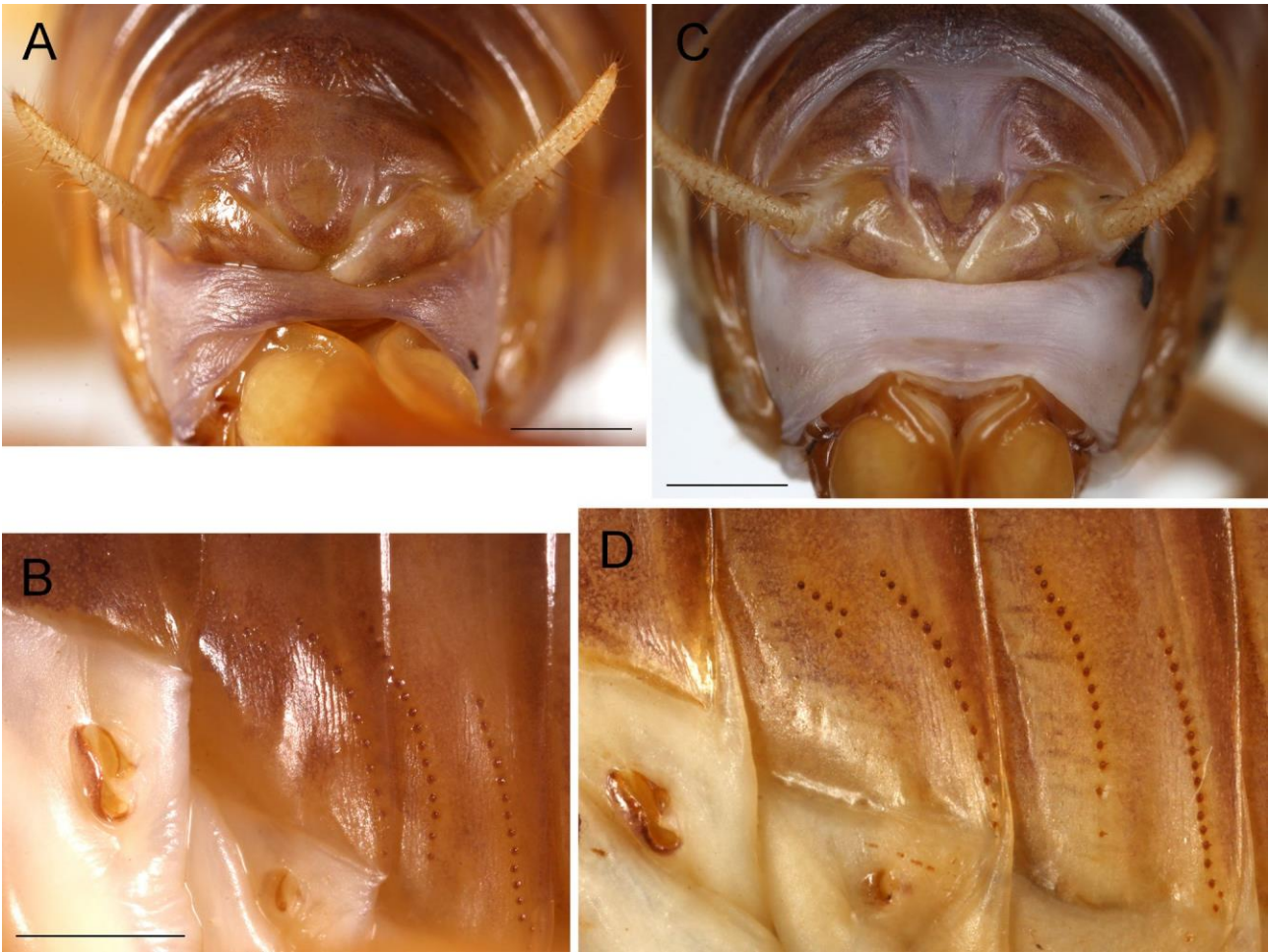
FIGURE 3. Monseremus appendiculatus (A, B) and Monseremus bellus (C, D): female abdominal apex in posterior view (A, C); female stridulatory files on second and third tergites (B, D). Scale bars: 1 mm.
