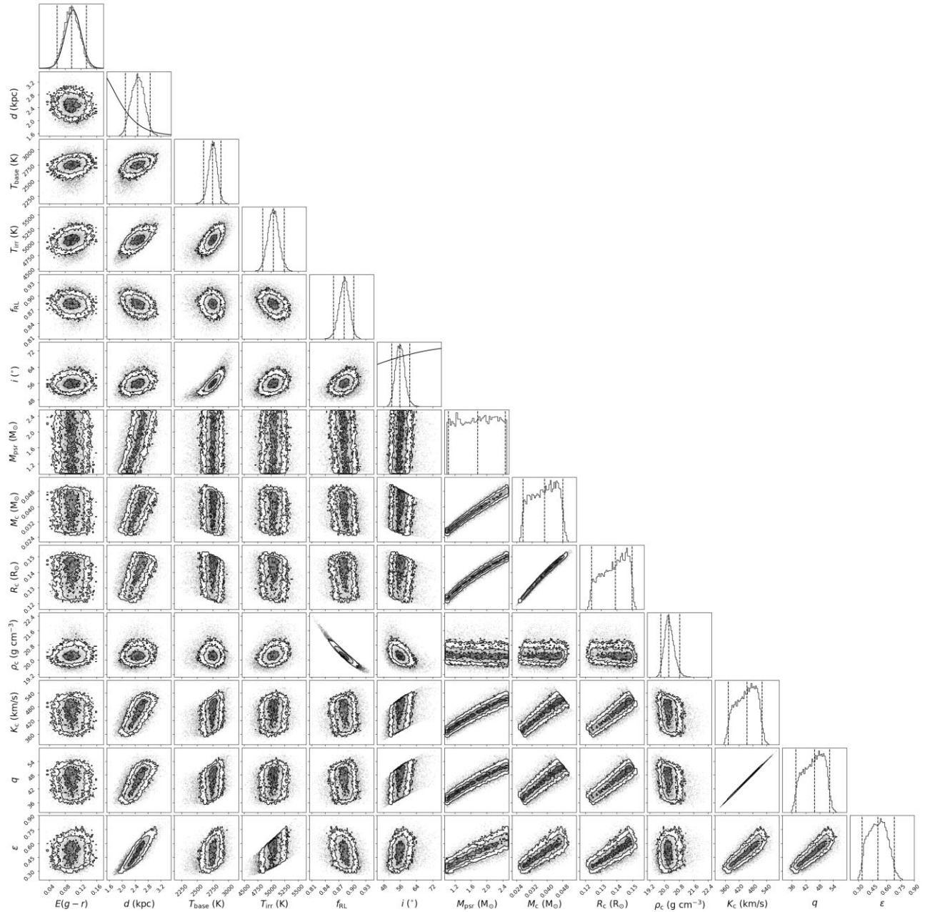
Figure 3. Corner plot showing the posterior distributions of the light-curve fit parameters. The last six parameters ( M_c , R_c , \rho_c , K_c , q , \epsilon ) were derived from the values of the fit parameters and the input parameters. The contours indicate the 1\sigma , 2\sigma , and 3\sigma confidence regions. The dashed vertical lines on the histograms show the mean and 95 per cent confidence intervals of the parameter distributions, and where non-uniform priors were used, these are shown as curves on the histograms.
