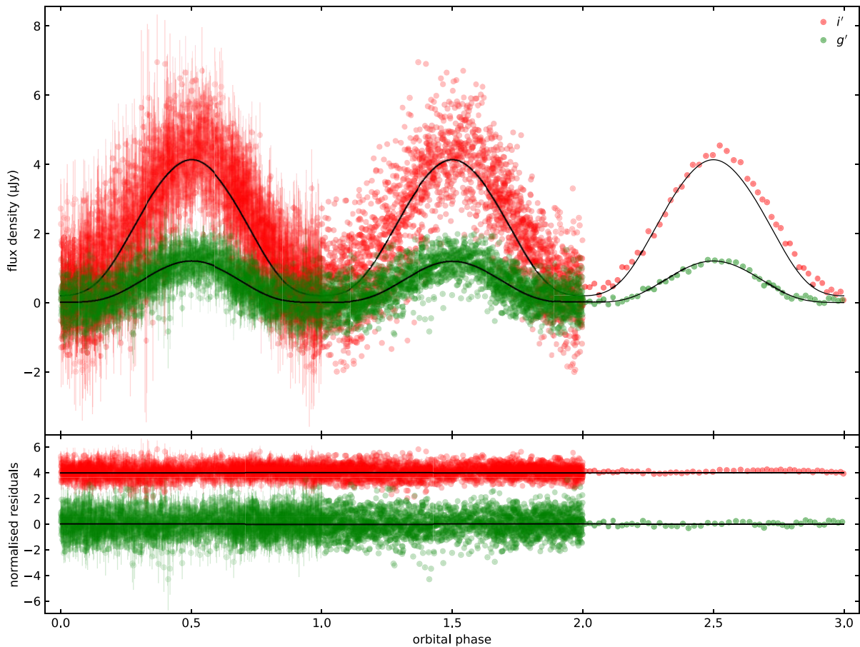
Figure 2. Upper panel: ULTRACAM g'i' light curves (green (bottom) and red (top) points, respectively) of PSR J2051–0827, phased according to the ephemeris given in equation (1). The folded light curve has been repeated three times, the first cycle with error bars, the second without, and the third cycle with every 45 data points binned, giving an effective exposure time of approximately 15 min per point. The solid lines show the result of fitting the HiPERCAM model presented in Fig. 1 to the ULTRACAM data, allowing only the flux scaling factors to vary. Lower panel: Normalized residuals of the ICARUS fits to the ULTRACAM data, offset vertically from each other by 4.0.
