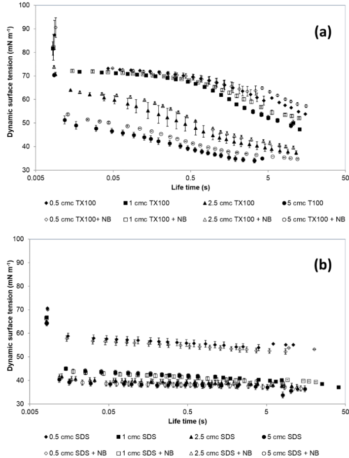
Figure 1 Dynamic Surface Tension results for the set of TX100 (a) and SDS (b) solutions from 0.5 (◆,◇), 1 (■,□), 2.5 (▲,△ and 5 cmc (●,○) described by filled symbols for surfactant solutions and by unfilled symbols for nanobubble-surfactant solutions. The error bars are standard errors.
