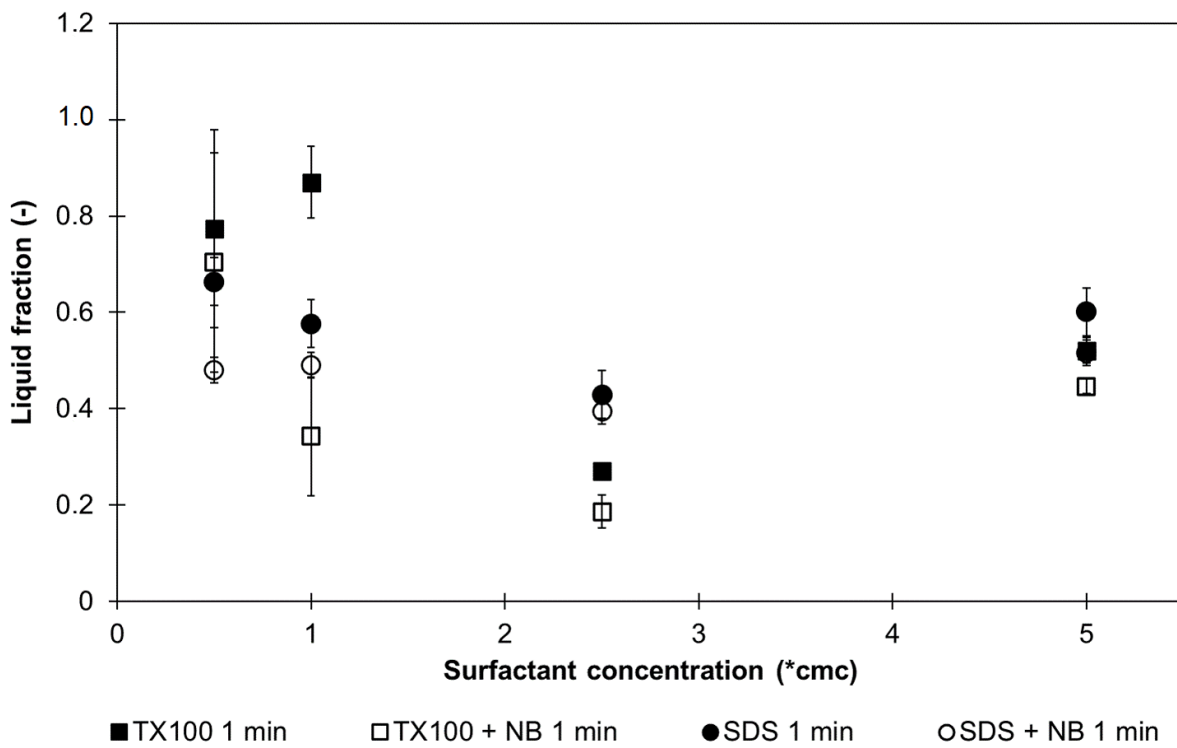
Figure 1 Foam liquid fraction evolution for Triton X-100 (square) and SDS solutions (circle) (filled symbols) versus bulk nanobubbles + Triton X-100 and bulk nanobubbles + SDS solutions (unfilled symbols). The error bars are standard errors.
