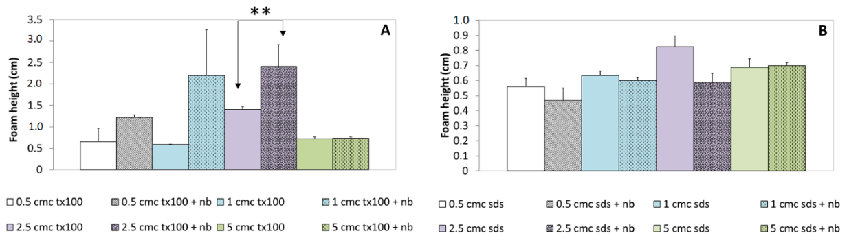
Figure 1 Initial foam heights after 1-minute foaming for 0.5 (white), 1 (blue), 2.5 (purple) and 5 (green) cmc Triton X-100 (A) and SDS solutions (B) (blank) versus bulk nanobubbles + Triton X-100 and SDS solutions respectively (symbols). The error bars are standard errors. Based on the ANOVA test, the asterisk “ ** ” means a p-value below 0.005.
