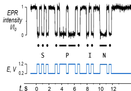
Fig. 4 Commutation of the EPR response of the TEMPO + /TEMPO redox couple immobilized at GC fibers ( \varnothing 5 \mu\text{m} ): the word “SPIN” written in inverted-key Morse code. Spin switching commands: E_{\text{OFF}}(“0”) = 1.2 V, E_{\text{ON}}(“1”) = 0.2 V, static field 3374 Gauss, and modulation amplitude 2 G. T = 293 K.
