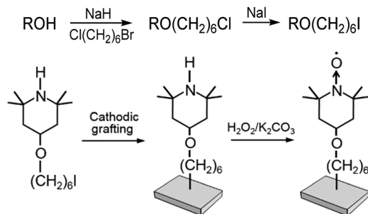
Scheme 1 Synthesis ( R = 4\text{-TMP} ), immobilization of \text{TMP-O(CH}_2)_6\text{I} and oxidation of the grafted \text{N-H} functions to \text{N} \rightarrow \text{O} .
