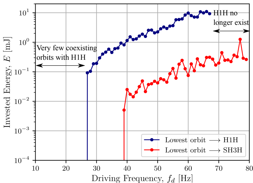
Figure 7: Evolution of the optimal invested energy required to jump from the lowest existing orbit to H1H (in blue) and those to jump from the lowest existing orbit to SH3H (in red) as a function of the vibration frequency.
