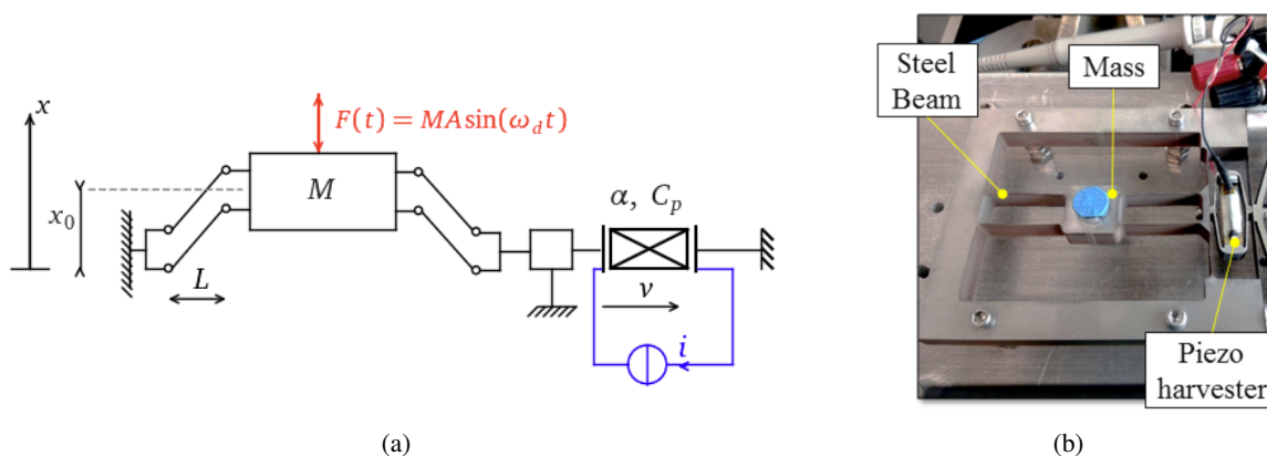
Figure 1: (a) Schematic of the vibration energy harvester (b). Experimental prototype of a Duffing-type VEH [8].
