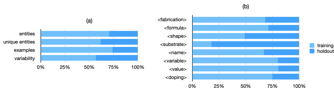
Figure 7. Holdout/training set for the Material ML model: (a) general metrics and (b) entity labels.
