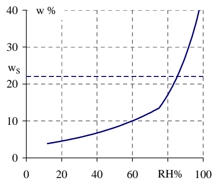
Fig. 1 Isotherm sorption curve of LVL material at the temperature T = 20^{\circ}C
