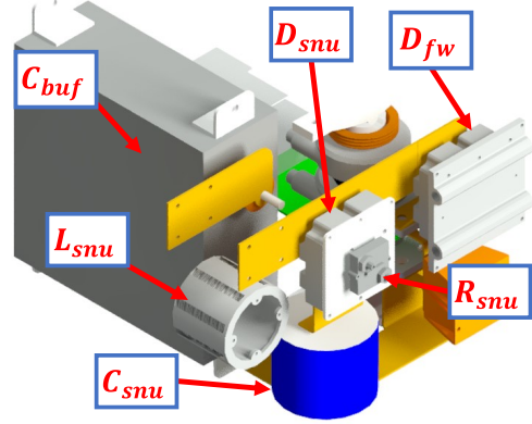
(b) Snubber side, with the cable inductor as the snubber inductor, 3D rendering (AutoCAD).
