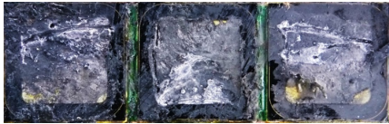
(c) Dies after snap-off destruction.
