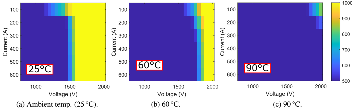
Fig. 8: Heatmaps representing the overvoltage level depending on voltage, current, and temperature during snap-off events. Diode used here: 4.5 kV diode. L_{snu}=3.4 \mu\text{H} .
