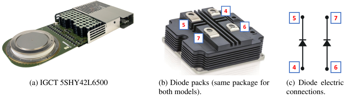
Fig. 3: Photograph of the selected semiconductor devices.
