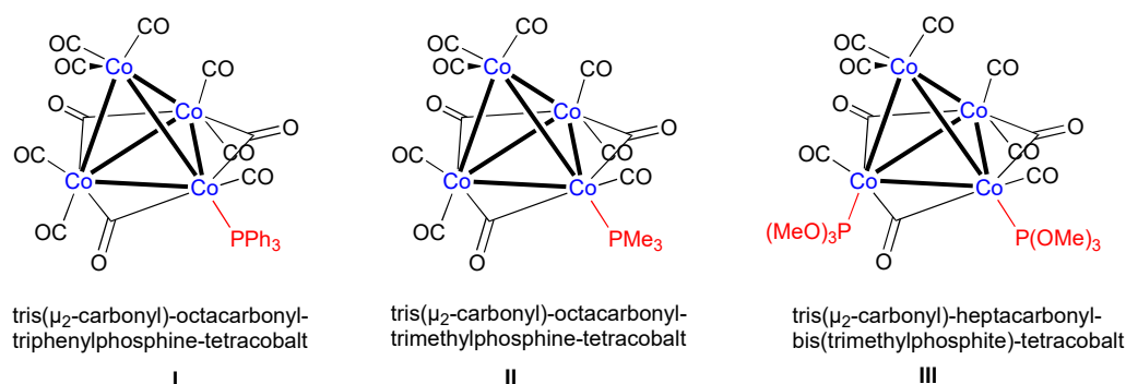
Scheme 1. Examples of some phosphine- and phosphite-substituted tetranuclear cobalt clusters [11,12].
