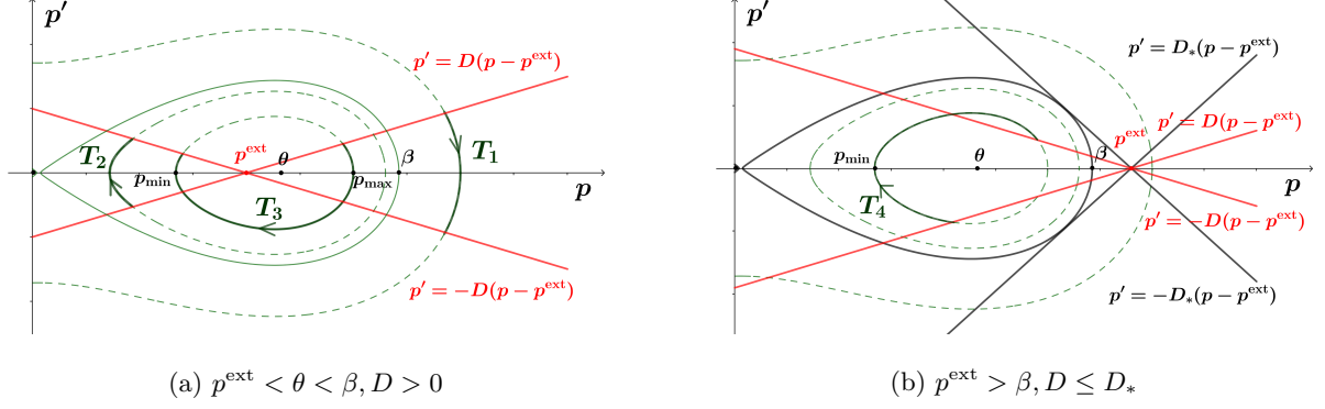
Figure 3: Phase portraits of (2): straight lines illustrate the boundary conditions, solid curves show relations between p' and p . Figure (a): curves T_1 , T_2 , and T_3 correspond to orbits of (SD), (SI), and non-(SM) solutions, respectively. Figure (b): curve T_4 corresponds to an orbit of a non-(SM) solution.
