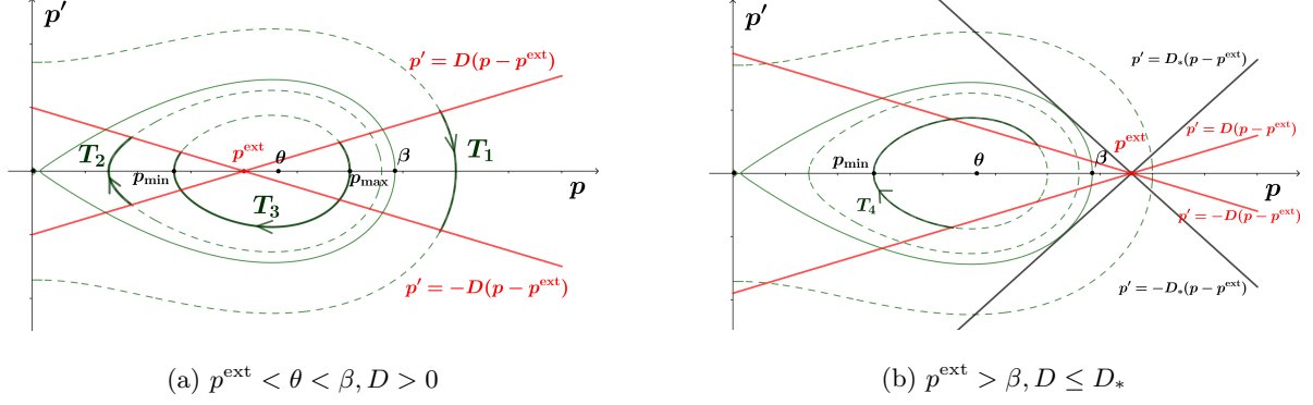
Figure 3: Phase portrait of eq. (2)
