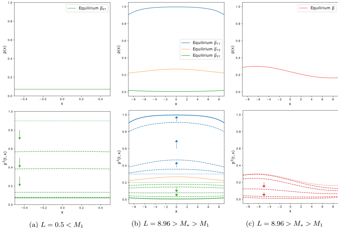
(a) L = 0.5 < M_1 (b) L = 8.96 > M_* > M_1 (c) L = 8.96 > M_* > M_1 Figure 6: Steady-state and time-dependent solutions when p^{\text{ext}} = 0.1, D = 0.05
