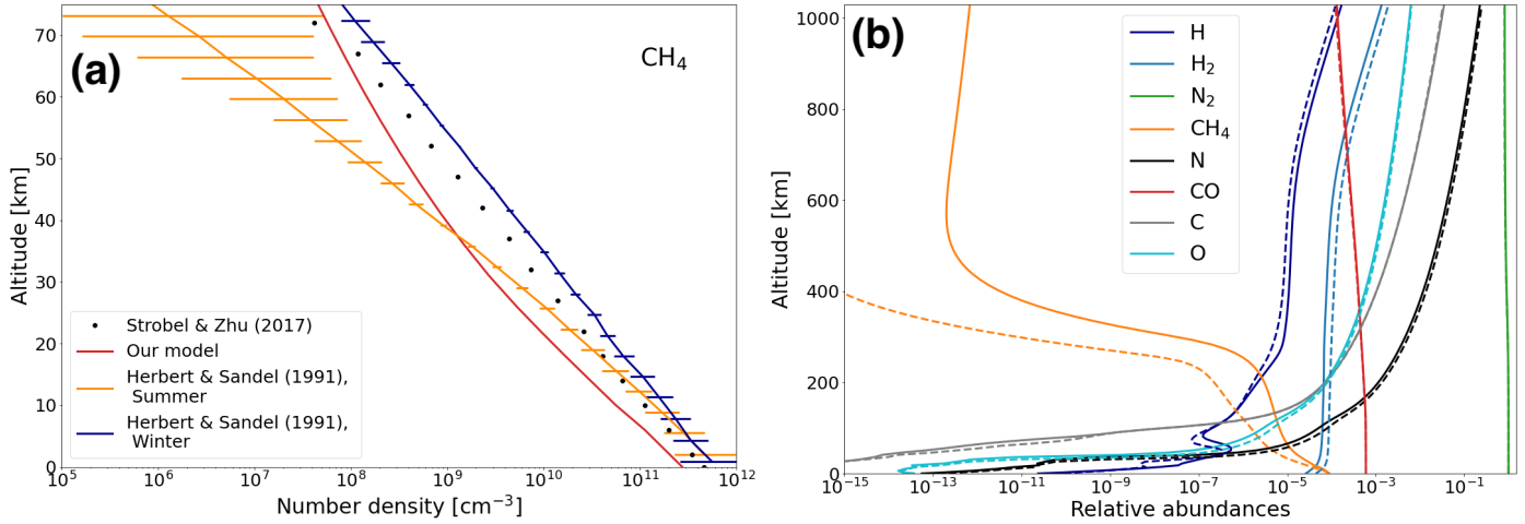
Fig. 9. Comparison of our CH 4 profile with other datasets and impact of the resolution of the solar spectrum on our results: (a) CH 4 number density profiles near the surface derived from Voyager 2 data and presented in Herbert & Sandel (1991) ; dark blue and orange), data points from Strobel & Zhu (2017) ; black dots) and result from our model using nominal reaction rates (red), i.e. without considering any uncertainty. (b) Comparison of the relative abundances of the main neutral species when using a high resolution solar spectrum (solid lines) versus a low resolution spectrum (dashed lines). These results are obtained with solar fluxes corresponding to low solar activity.
