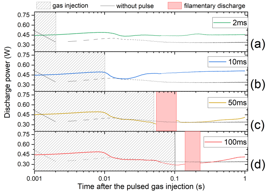
Figure 5: Discharge power (collected on the middle electrode) for various t_{gas} : (a) 2 ms, (b) 10 ms, (c) 50 ms and (d) 100 ms. Here, P_U is fixed to 2 bar. In the red zones, due to oscilloscope saturation in the filamentary regime, the power cannot adequately be calculated from current-voltage characteristics. A small drop is always observed for the first data point (only a few discharges in the 1-2 ms time scale); such a feature can be linked to the transition from filamentary to homogeneous discharge regime due to the time required for the buildup of the memory effect [47,49].
