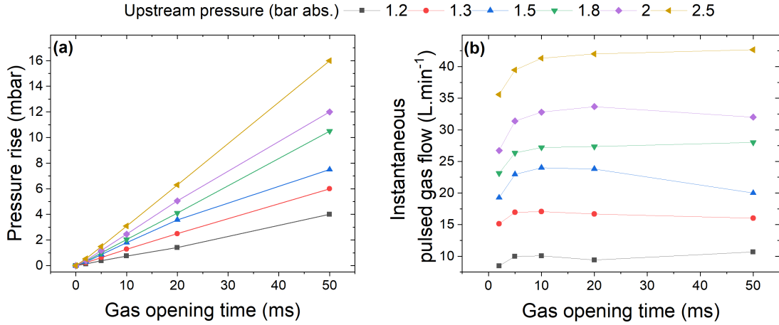
Figure 2: (a) Pressure variation ( \Delta P ) inside the closed chamber as a function of the gas opening time ( t_{gas} ) for various upstream pressures ( P_U ). Straight lines correspond to linear fits. (b) Instantaneous pulsed gas flow ( Q ) as a function of gas opening time for various upstream pressures ( P_U ). Lines are to guide the eye only.
