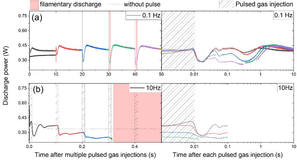
Figure 8: Discharge power for t_{\text{gas}} = 10 \text{ ms} at (a) 0.1 Hz and (b) 10 Hz injection frequency. The data are plotted over two-time scales: on a linear scale after multiple pulsed gas injections (left) and on a log scale after each pulsed gas injection (right). The same color code is used in both cases: black-first pulse, red-second pulse, blue-third pulse, green-fourth pulse and purple-fifth pulse.
