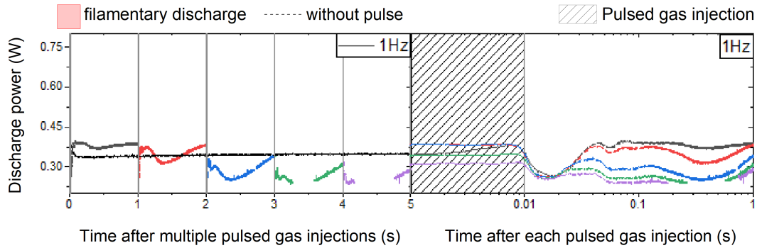
Figure 6: Discharge power for t_{\text{gas}} = 10 \text{ ms} , 2 bar. The data are plotted over two-time scales: on a linear scale after multiple pulsed gas injections (left) and on a log scale after each pulsed gas injection (right). The same colour code is used in both cases: black-first pulse, red-second pulse, blue-third pulse, green-fourth pulse and purple-fifth pulse.
