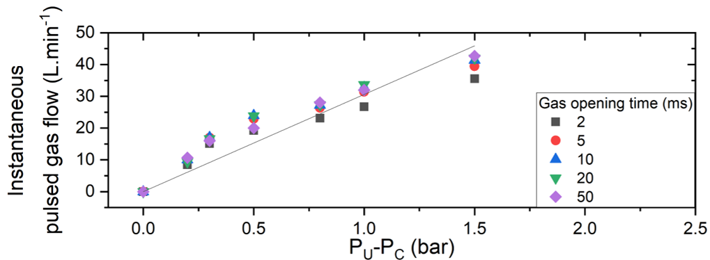
Figure 10: Correlation between the instantaneous pulsed gas flow Q and the pressure difference between the pulse injector and the chamber P_U - P_C for various gas opening times.
