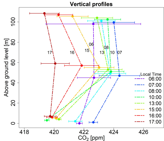
Figure 10. Vertical profiles from the eight pairs of flights. The ground level values are from the Picarro G2401 at CyI. CO 2 at 50 and 100 m a.g.l. are from the UAV CO 2 sensor horizontal flights; the error bars represent the standard deviation of the duration of each flight.
