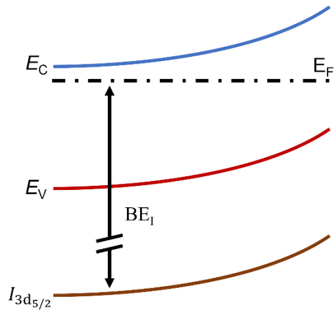
Figure 1: Sketch of the I_{3d_{5/2}} core level, top of the valence band, E_V , and bottom of the conduction band, E_C , in presence of a space-dependent electrostatic potential, q\varphi(x) = BE_1(x) = E_F - I_{3d_{5/2}}(x) .
