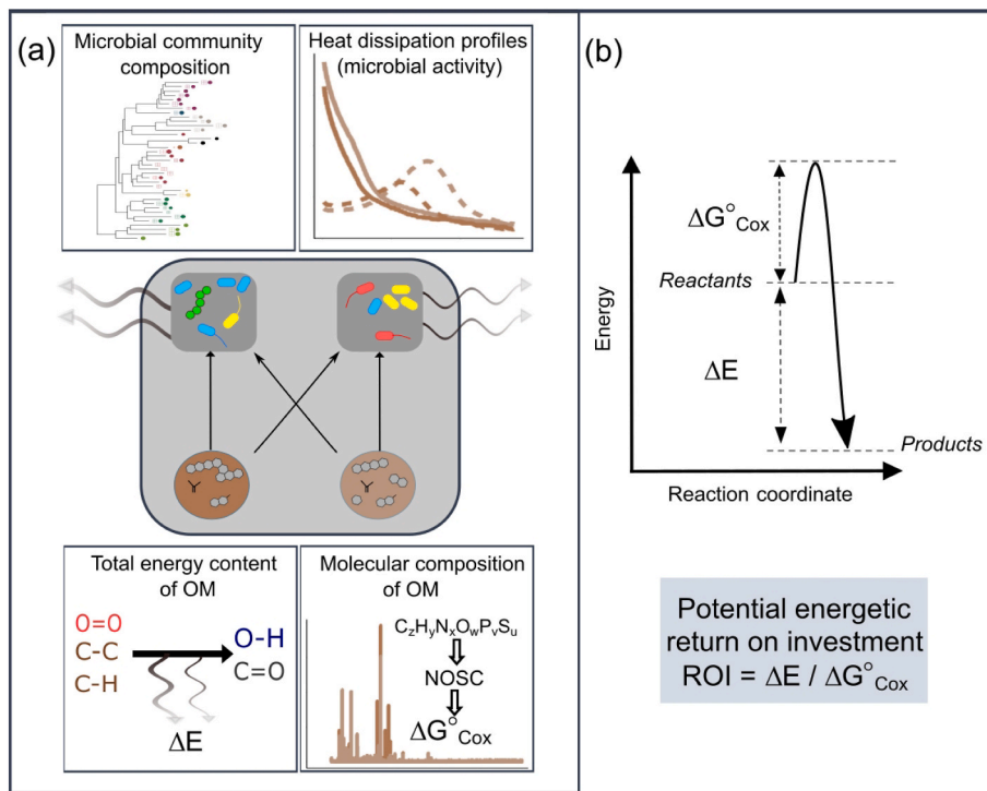
Fig. 1. Conceptual representation of the experimental design. (a) Six soil organic matter solutions containing different molecular profiles but the same quantity of organic C were added cross-wise to 6 soils (central panel). The soils harboured distinct bacterial communities (top left panel). The metabolic responses of microbial communities to the addition of soluble organic matter were determined as heat dissipation (wavy arrows) dynamics during a 24 h period (top right panel). The total energy content ( \Delta E ) was measured by bomb calorimetry (bottom left panel) and \Delta G^\circ_{Cox} was estimated from the molecular composition of substrates determined using Fourier transform ion cyclotron resonance mass spectrometry (bottom right panel). (b) The potential energetic return on investment (ROI) was calculated as the ratio between \Delta E and the weighted average \Delta G^\circ_{Cox} .
