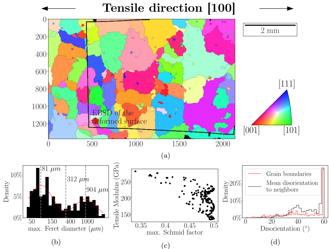
Figure 2: (a) Inverse Pole Figure (IPF) mapping (with regard to [001] direction) of the microstructure in the surface of interest that has been repositioned in the reference framework. Color coding is explained by the IPF unit triangle. Grains in black refer to unknown orientation. The area that was scanned again with EBSD after the test is delimited by the black lines. X and Y axes are expressed in pixels. (b) Corresponding bimodal grain size distribution (expressed by the maximum Feret diameter). (c) Maximum Schmid factor and Tensile modulus of all grains in the surface of interest. (d) Distribution of disorientation at grain boundaries and with respect to neighboring grains.
