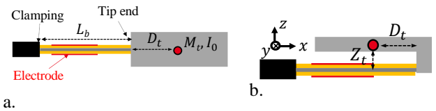
Fig. 1: a. Cantilever with conventional proof mass ( D_t > 0 ) b. cantilever with L-shaped proof mass ( D_t < 0 )
