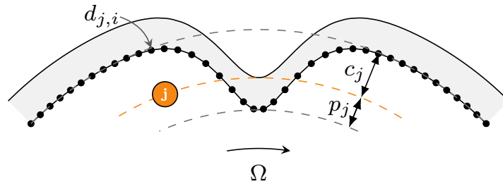
Figure 4. One lobe distortion of the casing (□) in front of the j -TH boundary node (●).
