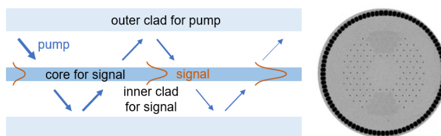
Figure 2. (Left) Illustration of double-clad fiber with step index profile. Center core for signal has highest index; inner cladding for the signal also guides the pump; outer cladding for the pump has the lowest index. (Right) Cross section of an advance large-mode-area photonic crystal fiber using air-holes in the low index regions. The center solid portion is the core for signal and the outer ring of air holes serves as the clad of the pump which guides pump in the fiber structure. It is designed for large-mode-area single-mode and polarization maintaining amplification, reprinted from Ref. [24]. See more about this technology in Sections 5.2 and 7.1.
