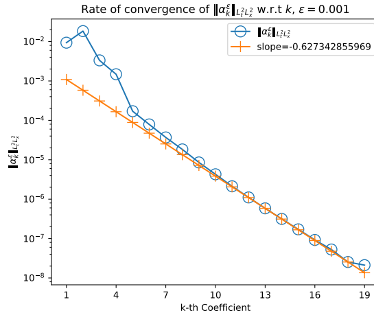
FIGURE 7. L_{t,x}^2 -norm of the Hermite coefficients of the solution of (1), as a function of k (log-scale) and for N_v = 20 , N_x = 28 , \Delta t = \varepsilon/35 , \varepsilon = 0.001 .
