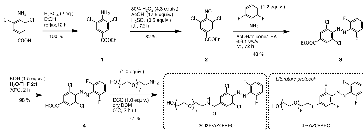
Scheme 1. Synthetic route for 2Cl 2 F-AZO-PEO, and the structure of 4F-AZO-PEO obtained according to the protocol reported by Huang et al. [14] The azobenzenes are drawn in their trans configurations.
