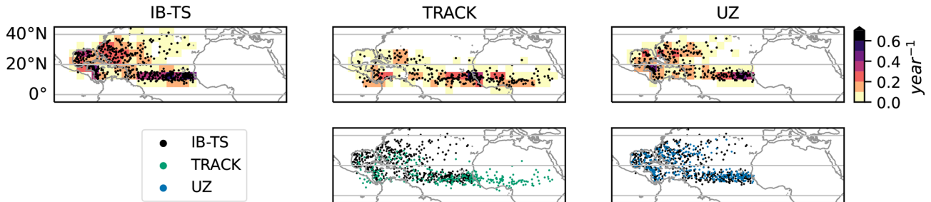
Figure 9. First observed/detected points in IB-TS, TRACK and UZ. Top row shows the first points along with the corresponding density. Bottom row overlays IB-TS tracks' first point with ERA5 tracks' first point as detected tracks by TRACK (second column) and UZ (third column).
