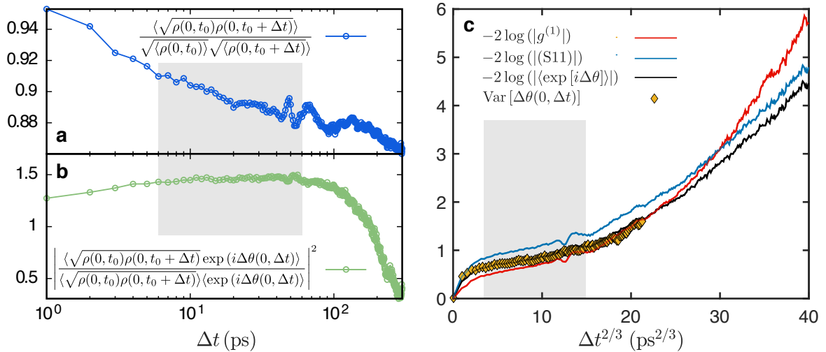
FIG. 17. a Density-density correlations. b Density-phase correlations. c Successive approximations of -2 \log(|g^{(1)}|) . The red line is the full reconstruction of -2 \log(|g^{(1)}|) , taking into account phase-phase, density-density and density-phase correlations. The blue one is obtained from Eq. (16), neglecting density-phase correlations in g^{(1)} . The black line shows the variations of -2 \log(|\langle \exp(i\Delta\theta) \rangle|) where density-density and density phase correlations are neglected. The grey shaded region in all panels indicates the KPZ window.
