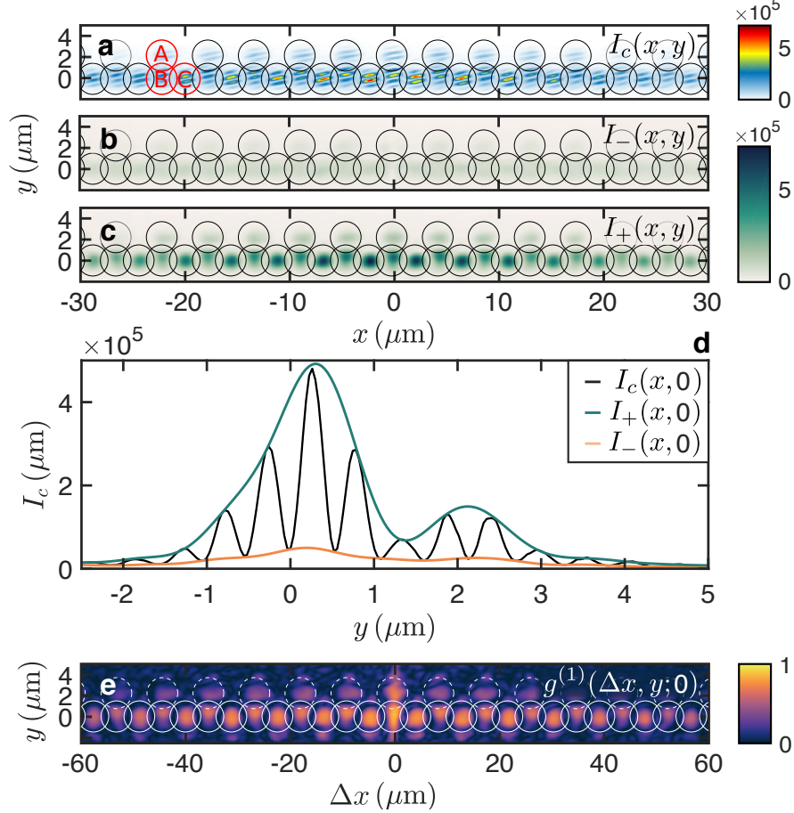
FIG. 8. Retrieving the first order coherence of polariton condensates. a Interference pattern captured by the CCD for \Delta t = 0 . b-c lower and upper envelopes of the interferogram. d Cut of the first three maps along x = 0 . Coherence retrieved from Eq. (27). The photoluminescence background strongly interferes with itself at (\Delta x = 0, \Delta t = 0) , creating a peak in |g^{(1)}| at \Delta x = 0 . This peak disappears after one scan step only, as the photoluminescence background light is fully incoherent.
