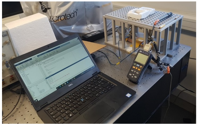
Fig. 7. Photo of the measurement bench and tags.
