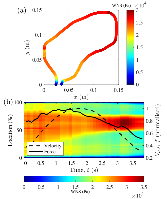
Fig. 3: a: Instantaneous variations of the wall normal stress (WNS) along the boundaries of the rectum at t = 0.5 s. The color code corresponds to the magnitude of WNS. b: Spatio-temporal map of WNS along the boundaries of the rectum. The location 0 and 100 % correspond to the anterior and posterior part of the anus, respectively. Plain and dashed lines show respectively the temporal variations of the magnitude of the force \vec{f} and the outlet velocity V_{out} , which are scaled by their maximal value (right y -axis).
