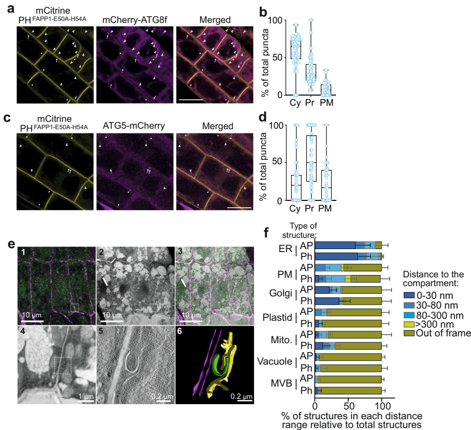
Fig. 7 | Autophagy structures form close to PI4P-enriched compartments. a–d Confocal images of 7-day-old seedlings co-expressing the PI4P-binding probe mCititrine-1xPH FAPP1-E50A-H54A and either mCherry-ATG8f ( a ) or ATG5-mCherry ( c ). Plants were placed in autophagy induction conditions (–NC) for 1.5 h. Empty arrowheads indicate puncta in the cytosol (Cy), full arrowheads indicate puncta at proximity from the plasma membrane (Pr) and arrows indicate puncta on the plasma membrane (PM). Scale Bar: 10 \mu m. Repartition of the three distinct types of ATG8 or ATG5 puncta populations are presented in b and d , respectively. For each image we counted the total number of puncta as well as the number of puncta in each category. We used these data to calculate the percentage of puncta in each category compared to total puncta. Box plots indicate all individual values and median (middle line), 25th, 75th percentile (box), and 5th and 95th percentile (whiskers). In b , n = 52 images were examined over four independent biological experiments; in d , n = 49 images were examined over 5 independent biological experiments. e (1) Confocal acquisition of the root tip of seedlings co-expressing GFP-ATG8a and 2xmCherry-2xPH FAPP1 after 1.5 h induction of autophagy using 1 \mu M
